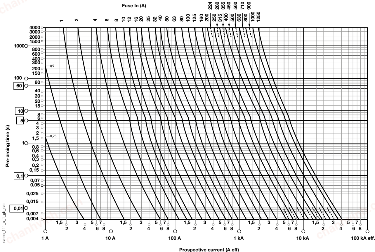
Time/current operation characteristics
