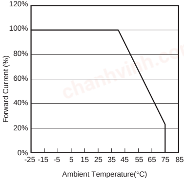
Fig.8 Derating
