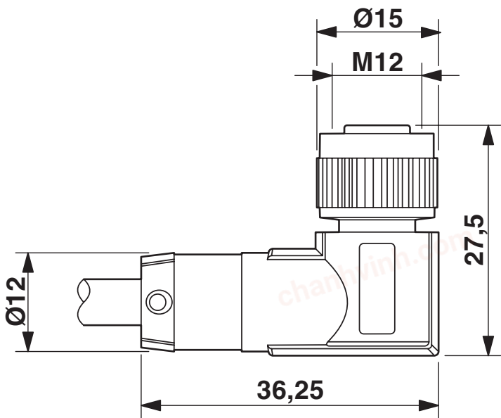
Dimensional drawing
