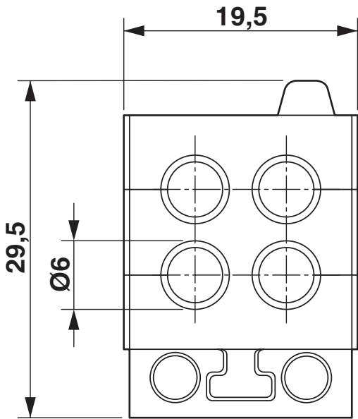
Dimensional drawing
