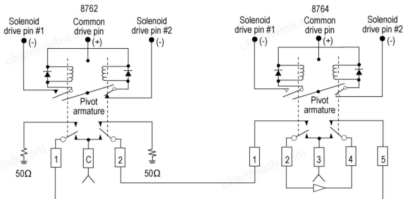
Figure 6. Signal reversal
