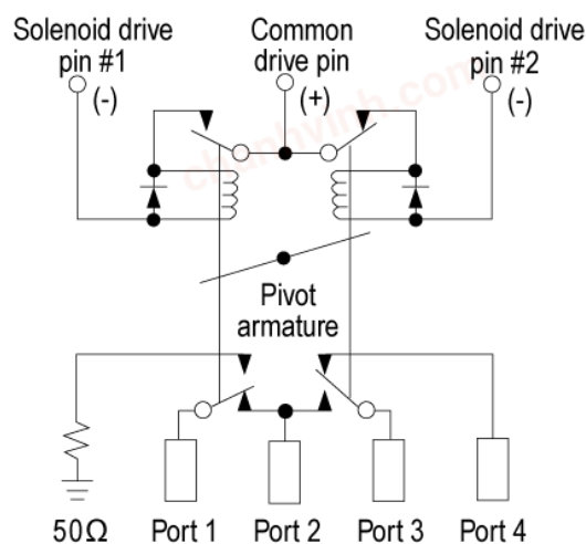
Figure 2. Keysight 8763
