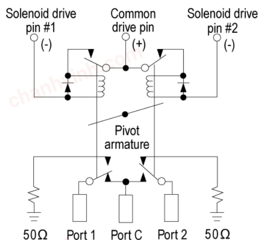
Figure 1. Keysight 8762
