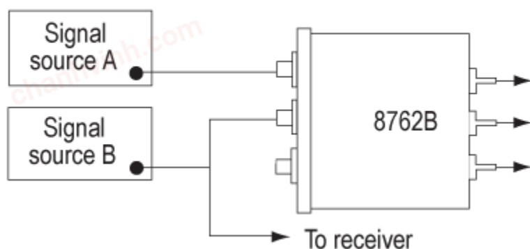
Figure 4. Multi-source switching
