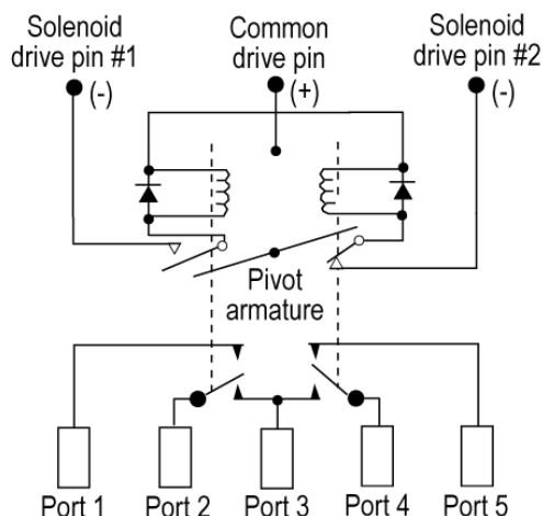
Figure 3. Keysight 8764
