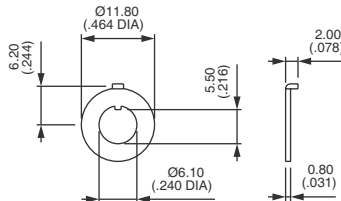
LOCKING RING
