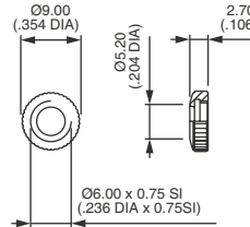
KNURLED CAP NUTS
