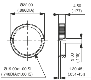
KNURLED NUT FOR MODELS Ø 19 (.748)
