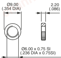
KNURLED NUT
